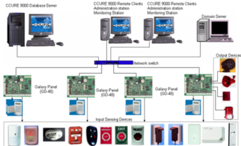
Figure 1: Galaxy Intrusion Integration Architecture
